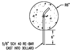
3 SECTION VIEW
